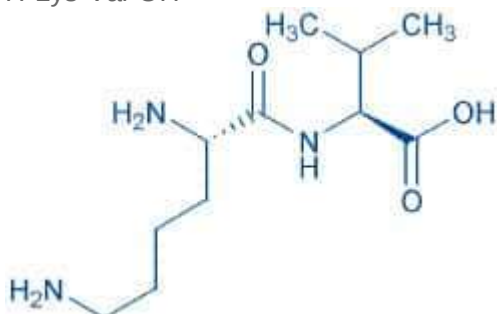
H-Lys-Val-OH
