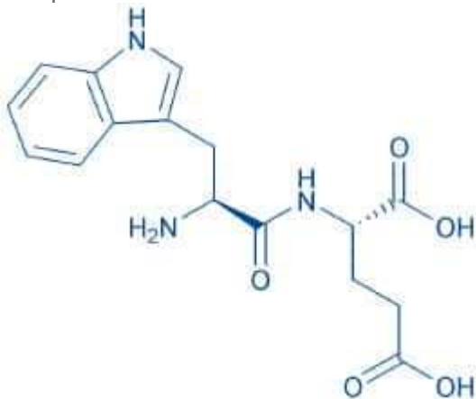
H-Trp-Glu-OH
