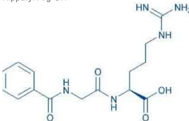
Hippuryl-Arg-OH
