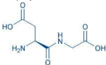
H-Asp-Gly-OH
